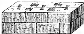
Fig. 269. Dove-tailed Masonry.
